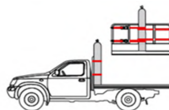
3. Tanks correctly fastened in a vertical position.
