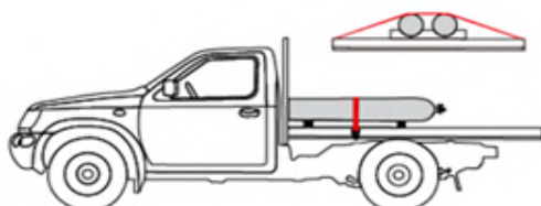
4. Tanks correctly fastened in a horizontal position. It is not recommended to transport liquefied gases in a horizontal position
